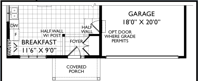
PARTIAL GROUND FLOOR PLAN EL. 'B'
