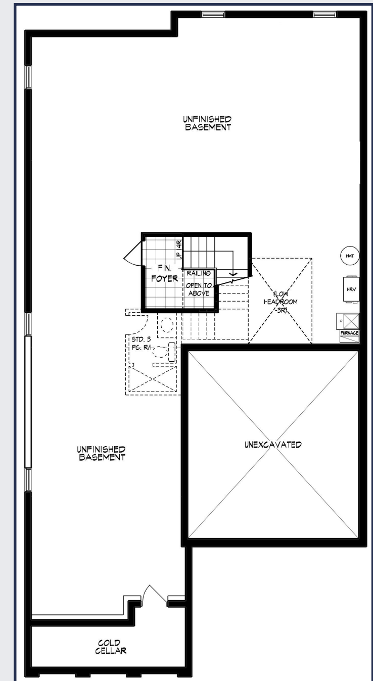
BASEMENT PLAN, EL. 'A'
