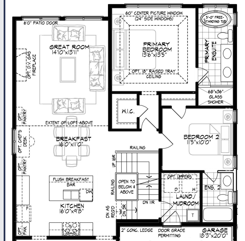
PARTIAL GROUND FLOOR PLAN, EL. 'B'
