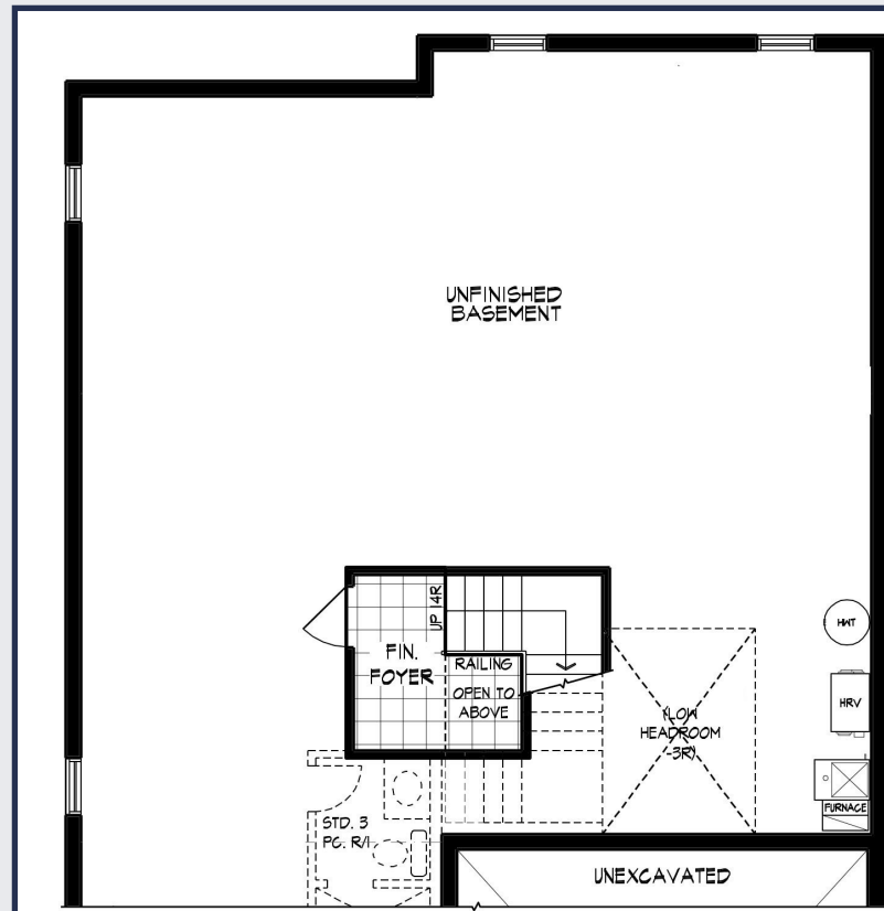
PARTIAL BASEMENT PLAN, EL. 'B'
