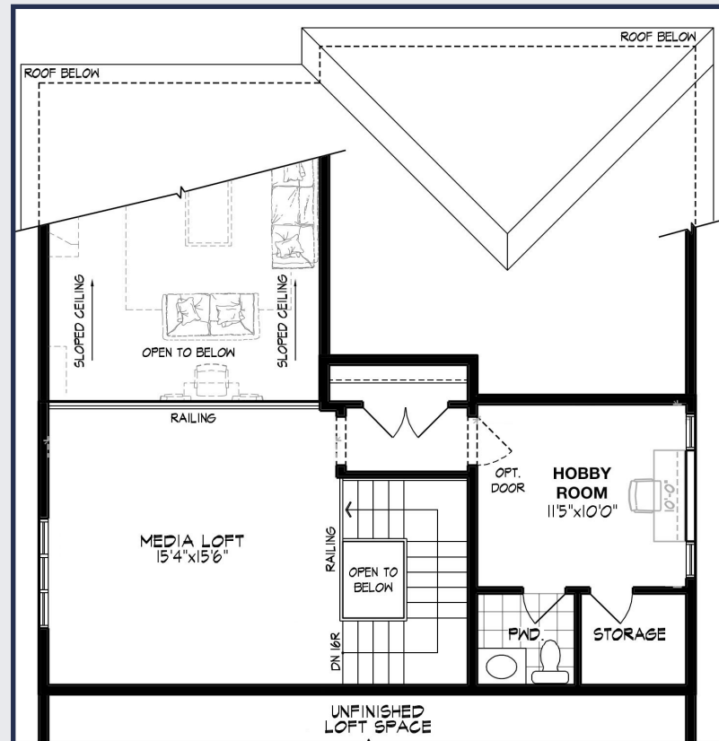
PARTIAL LOFT FLOOR PLAN, 'B'
