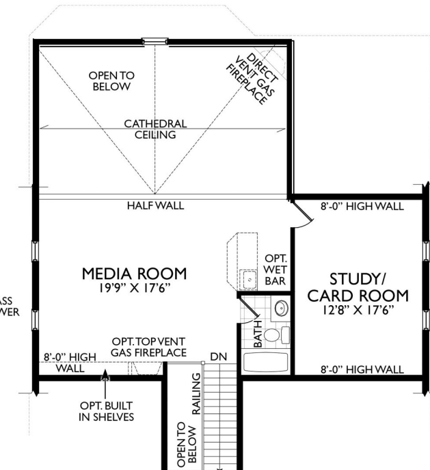
LOFT FLOOR PLAN EL. 'A', 'B' & 'C'
