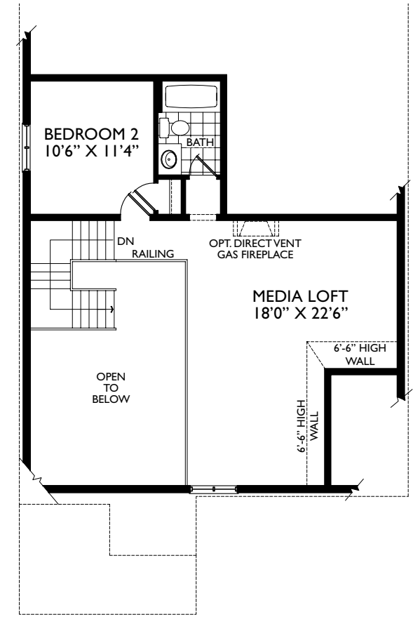
LOFT FLOOR PLAN EL. 'A'
